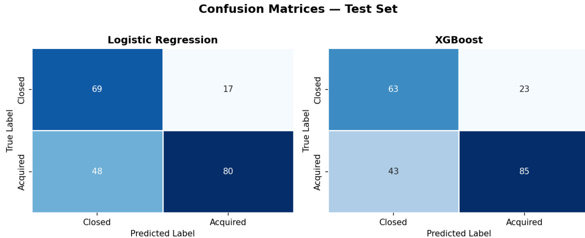
Figure 2: Confusion matrices for Logistic Regression (left) and XGBoost (right). XGBoost identifies more true acquisitions (85 vs 80) at the cost of slightly more false positives among closed startups.
